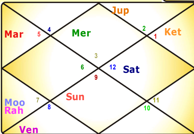
Asttotari-Amsha Chart
