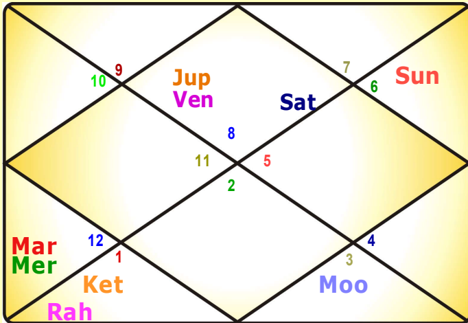
Dwisaptati-Amsha Chart
